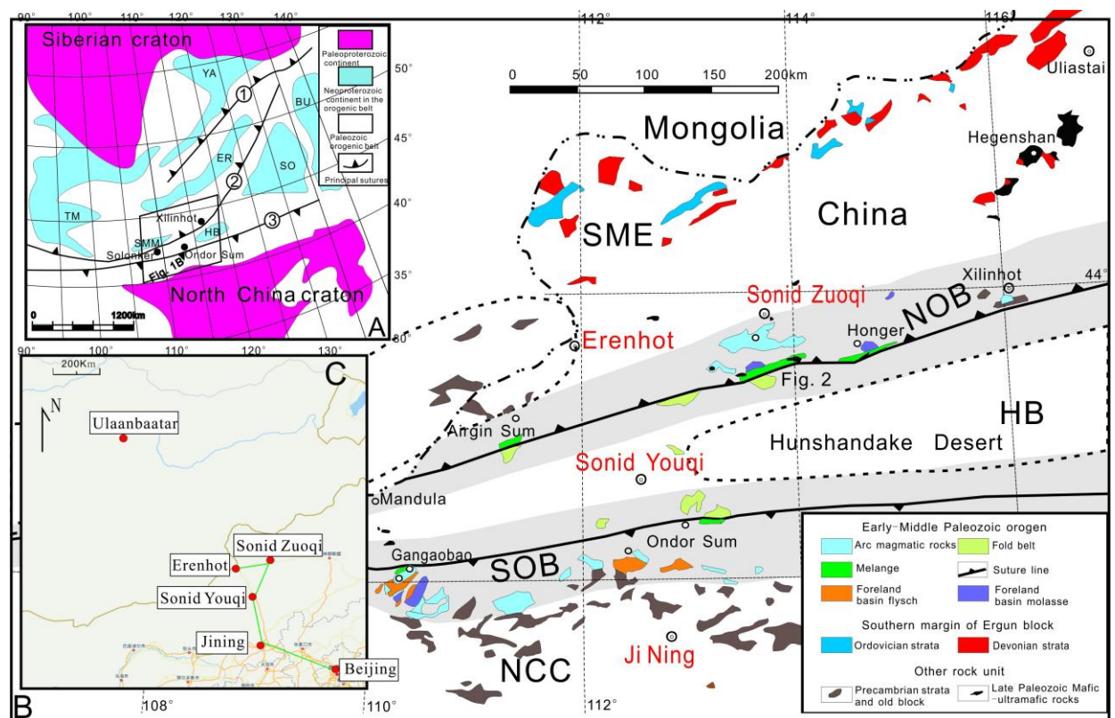
Fig. 1. Tectonic map showing location of the field excursion
